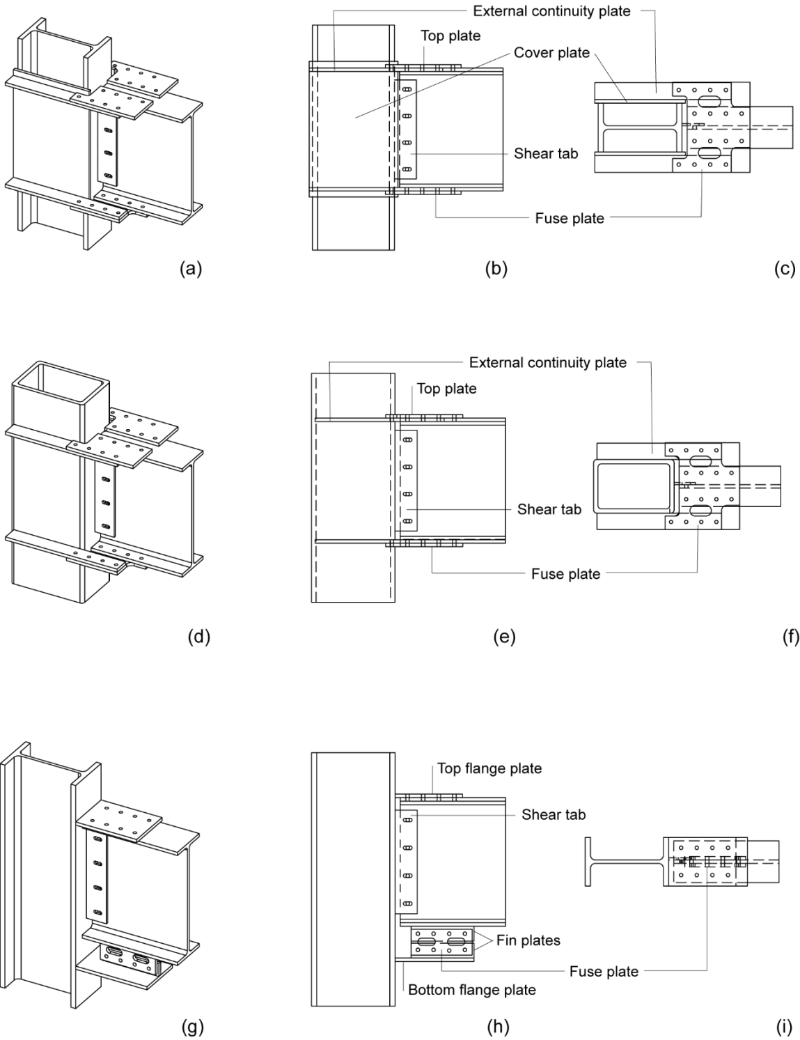
FIGURE 1 – DURAFUSE FRAMES CONNECTION
